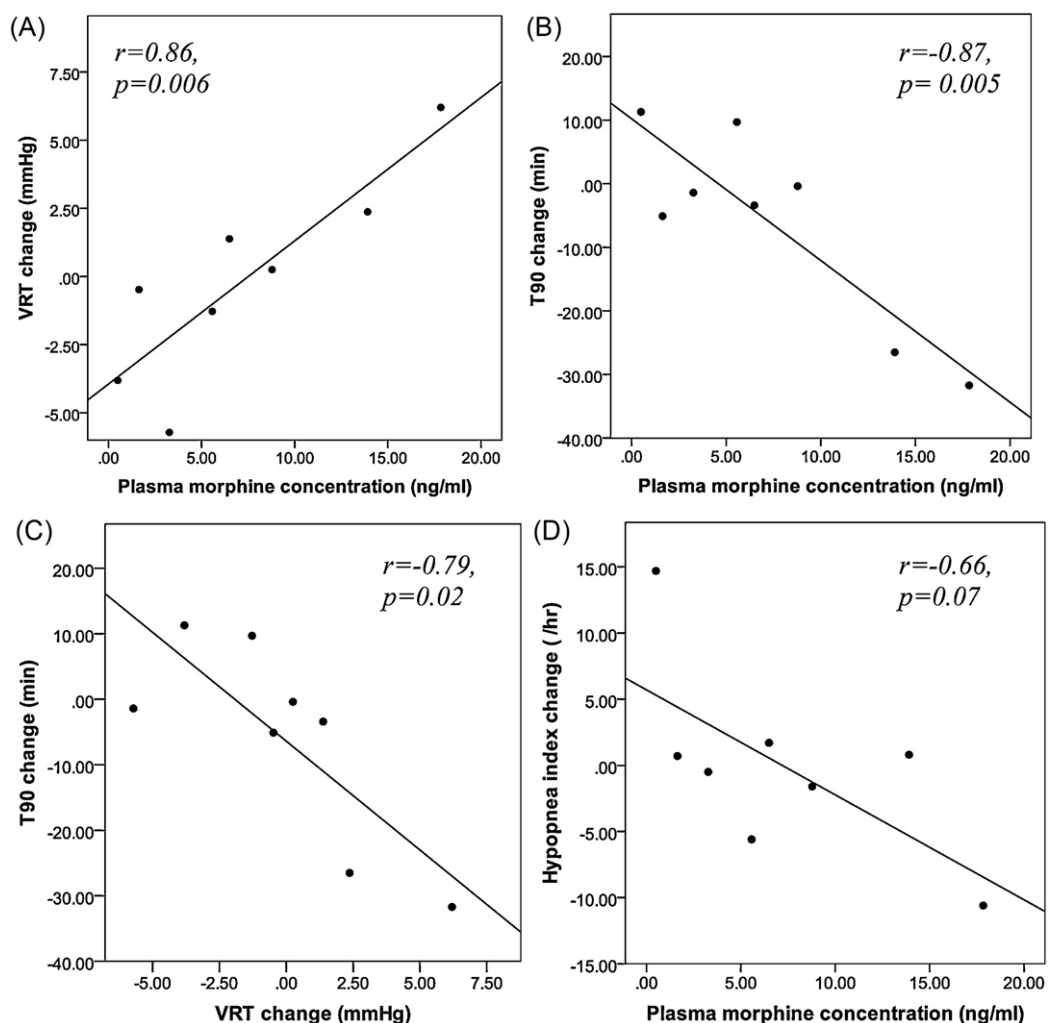
Fig. 2. Between the morphine arm and baseline, significant associations were found between individual plasma morphine concentration and the change of awake VRT (Panel A), and the change of Sleep Time with Sp_{O_2} < 90\% (T90) (Panel B). Panel C shows the association between the change of VRT and the change of T90 min. Panel D shows that a higher plasma morphine concentration tended to correlate with an improvement in hypopnoea index compared to the baseline. The changes were calculated by (morphine arm – baseline).
